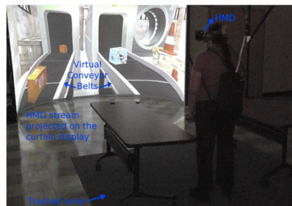
Figure 2: The user is looking at the virtual conveyor belts. View of the user inside the HMD is projected on a curtain display, only for outside viewing purposes. The lights in the room are turned off to prevent any light bleeding inside the headset.
